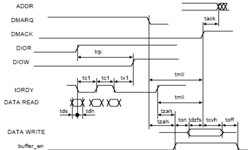
Figure 69. UDMA in Host Terminates Transfer Timing Diagram
