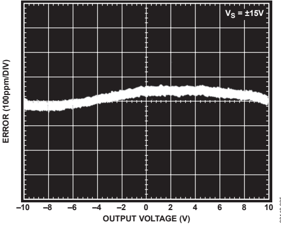
Figure 26. Gain Nonlinearity, G = 1000 , R_L = 10 k\Omega
