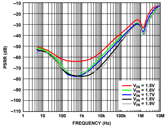
Figure 32. Power Supply Rejection Ratio (PSRR) vs. Frequency at Various Input Voltages ( V_{in} ), V_{out} = 1.3 V, Load = 5 A
