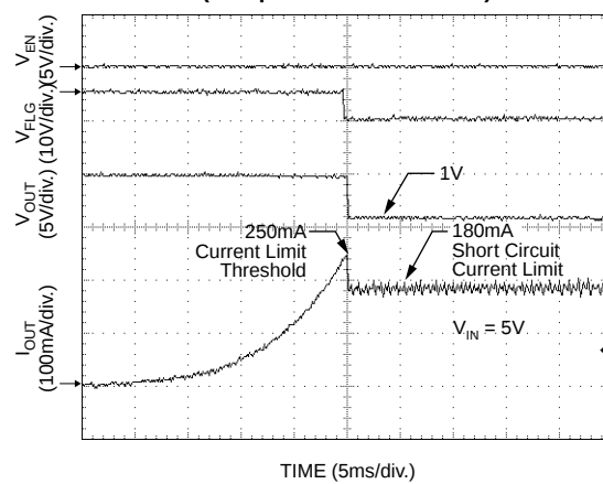
Current Limit Response (Ramped Load: MIC2537-2)
