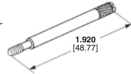
4-40 Male Jackscrew Kit Nos.: 747784-8 (bulk packed)*†
