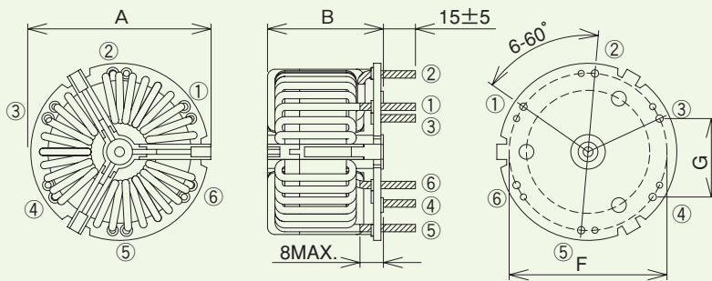
Figure 34. FM□□K□□□MBPF
