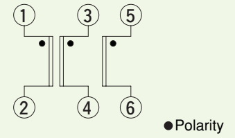
Figure 35. Circuit diagram
