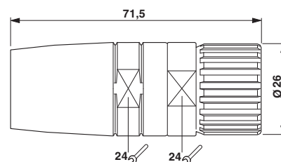
Dimensional drawing
