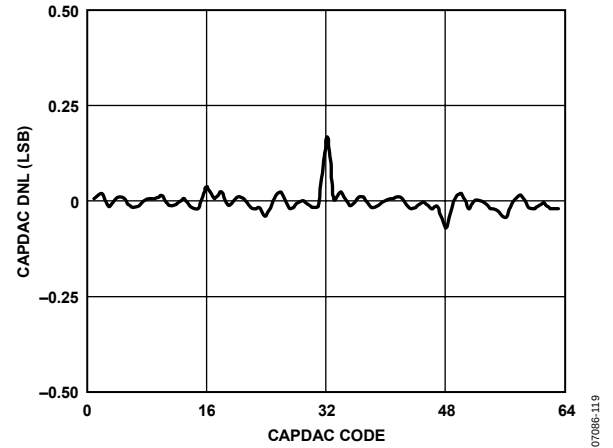
Figure 19. CAPDAC Differential Nonlinearity (DNL), V_{DD} = 3.3\text{ V}
