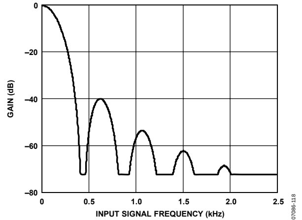
Figure 18. Capacitance to Digital Converter Frequency Response
