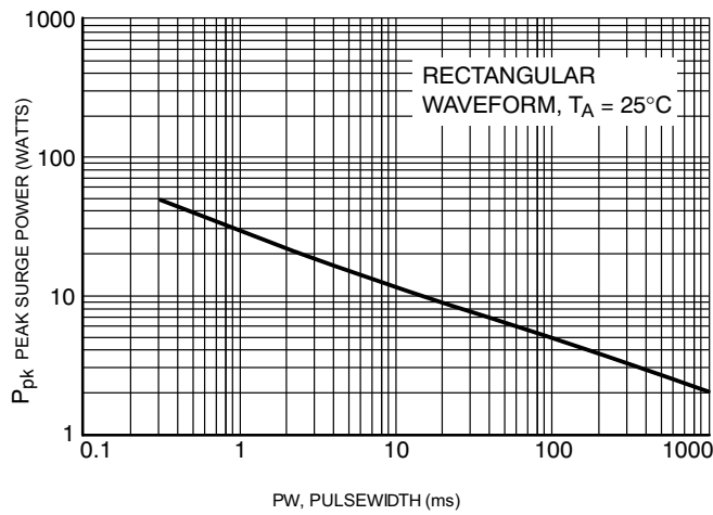
Figure 9. Maimum Nonrepetitie Surge Power
