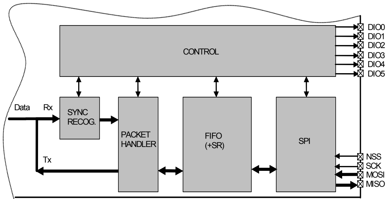
Figure 23. Packet Mode Conceptual View
