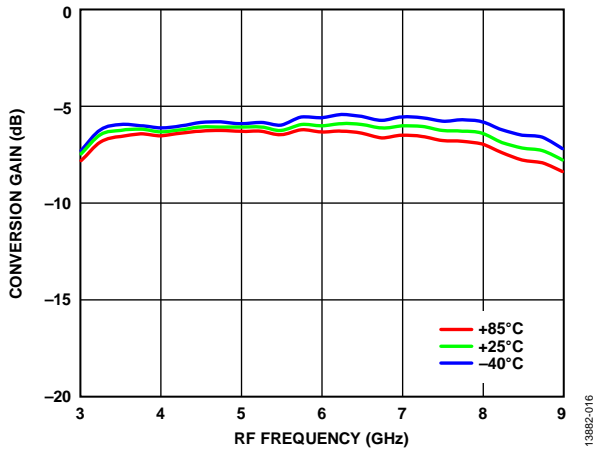
Figure 16. Conversion Gain vs. RF Frequency at Various Temperatures, LO = 15 dBm
