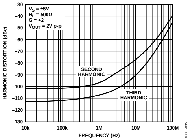
Figure 35. AD9632 Harmonic Distortion vs. Frequency, R_L = 500\Omega
