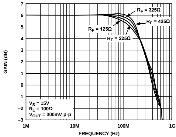
Figure 29. AD9632 Small Signal Frequency Response, G = +2
