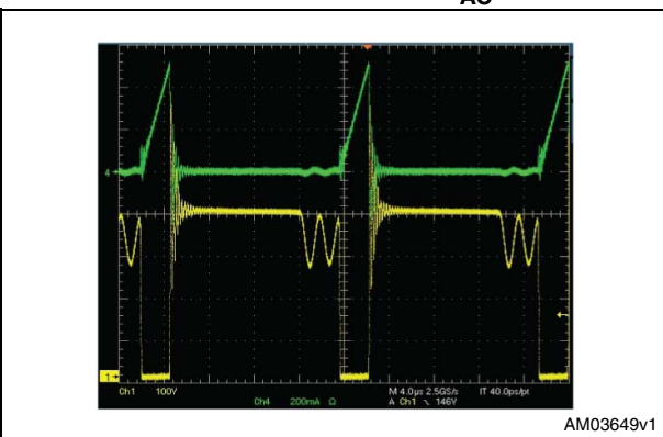
Figure 8. Drain current and voltage at maximum load 230 V AC
