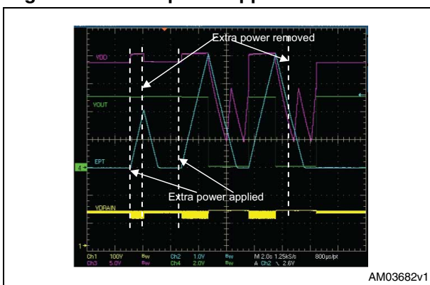
Figure 42. Extra power applied and removed
