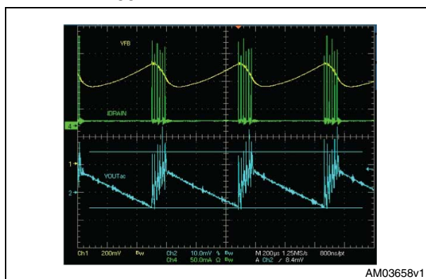
Figure 17. Output voltage ripple at 115 V IN_AC 50 mA
