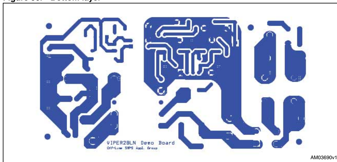
Figure 50. Bottom layer
