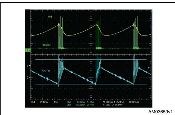
Figure 18. Output voltage ripple at 230V IN_AC 50 mA
