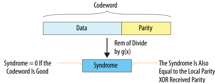
Figure 4-10: Codewords, Parity and Syndromes
