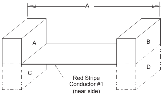
Left Connector
