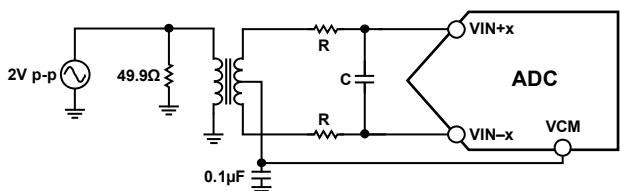
Figure 42. Differential Transformer-Coupled Configuration
