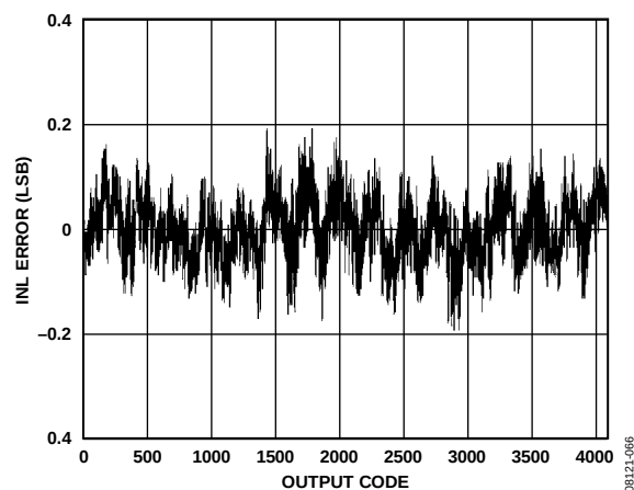
Figure 17. AD9231-80 INL with f_{IN} = 9.7 MHz
