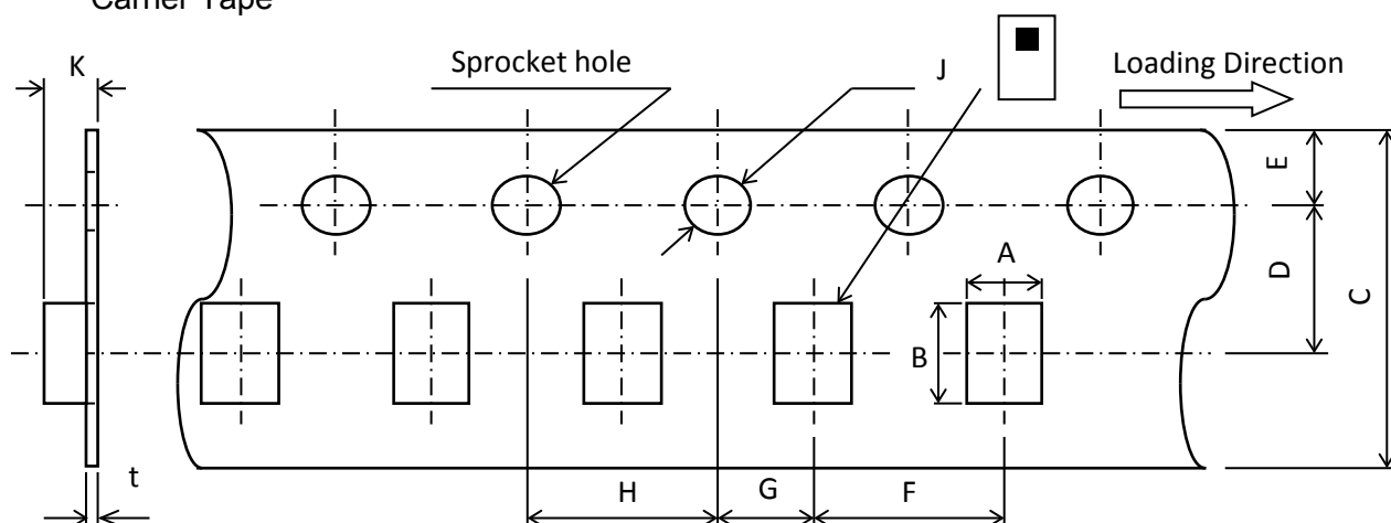
Carrier Tape
