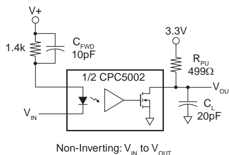
Figure 2. Non-Inverting Configuration
