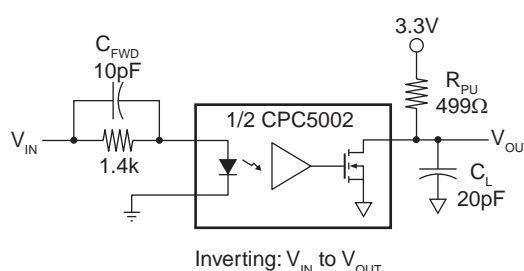
Figure 1. Inverting Configuration
