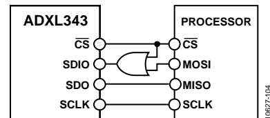
Figure 26. Recommended SPI Connection Diagram when Using Multiple Devices on a Single Bus
