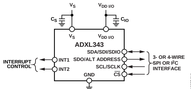
Figure 34. Application Diagram
