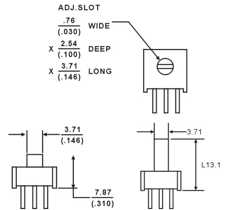
TSR-3386(STYLE)-EY5-(RESISTANCE CODE)-T The Model 3386 is available with a knob for finger adjustment. Add suffix letter "T" to order code.
