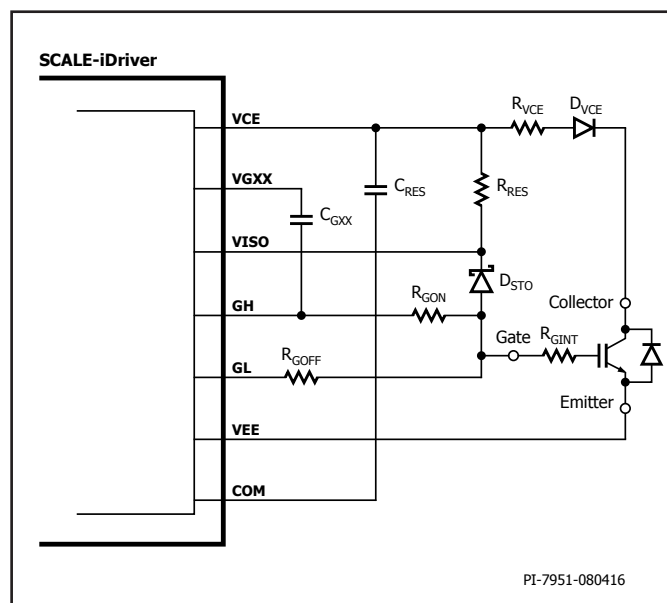
Figure 9. Short-Circuit Protection Using Diode D_{VCE} .
