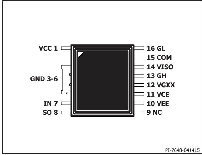
Figure 4. Pin Configuration.
