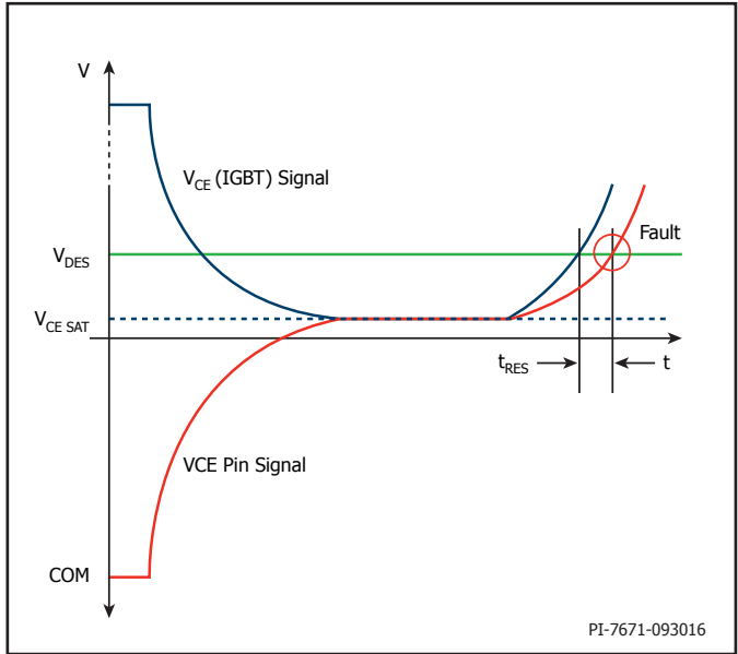
Figure 11. Short-Circuit Protection Using Resistor Network R_{VCE*}
