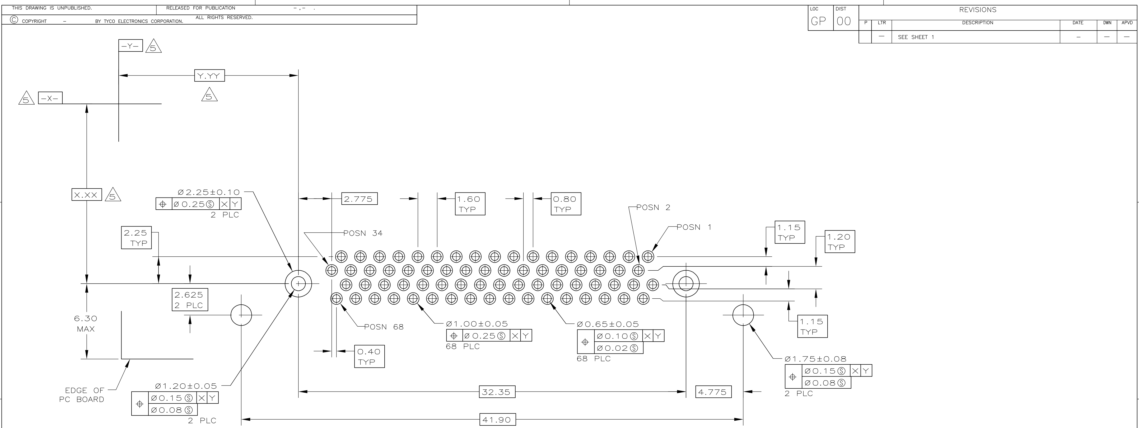
PC BOARD MOUNTING DIMENSIONS 3
