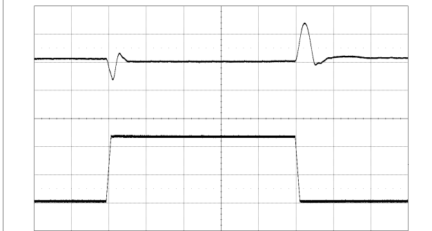
Output Load Transient Response, Default Configuration
