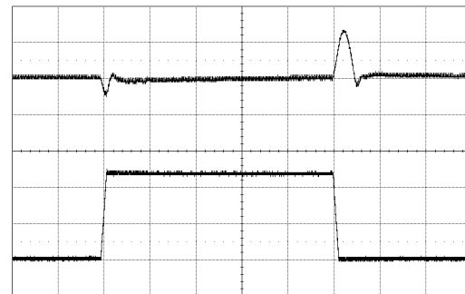
Output voltage response to load Step-change (12.5-37.5-12.5 A) at: T_{P1} = +25^\circ C , V_I = 12 V , V_O = 1.0 V di/dt = 2 A/\mu s , f_{sw} = 320 kHz C_O = 470 \mu F /10 m \Omega Top trace: output voltage (200 mV/div.). Bottom trace: load current (10 A/div.). Time scale: (0.1 ms/div.).
