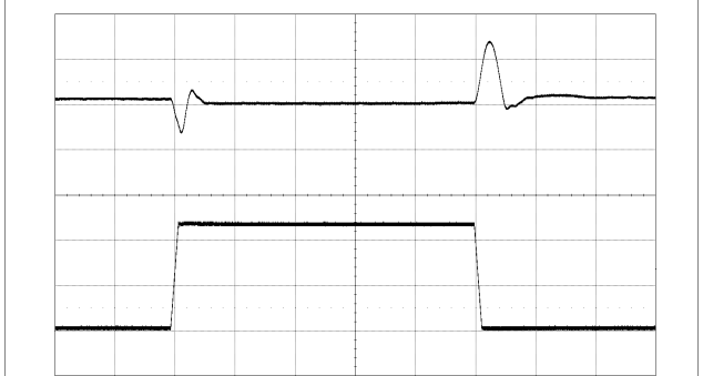
Output voltage response to load current Step-change (12.5-37.5-12.5 A) at: T_{P1} = +25\text{ }^\circ\text{C} , V_I = 12\text{ V} , V_O = 1.0\text{ V} di/dt = 2\text{ A}/\mu\text{s} , f_{sw} = 320\text{ kHz} C_O = 470\text{ }\mu\text{F}/10\text{ m}\Omega
