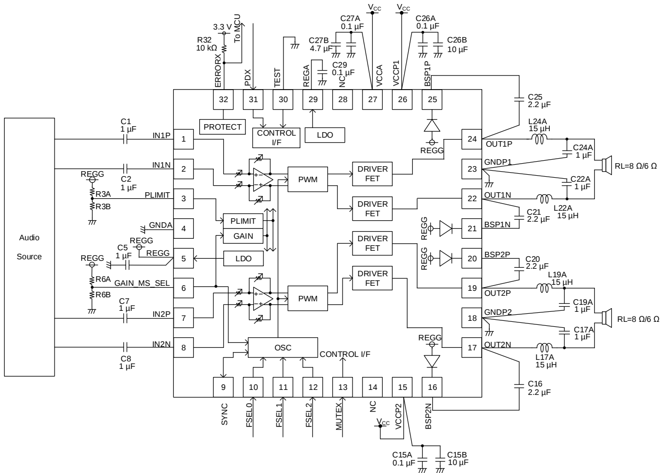
Figure 44. Application Circuit 1
