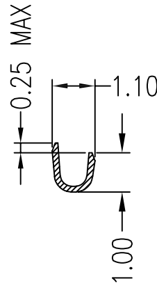
SEC B-B
