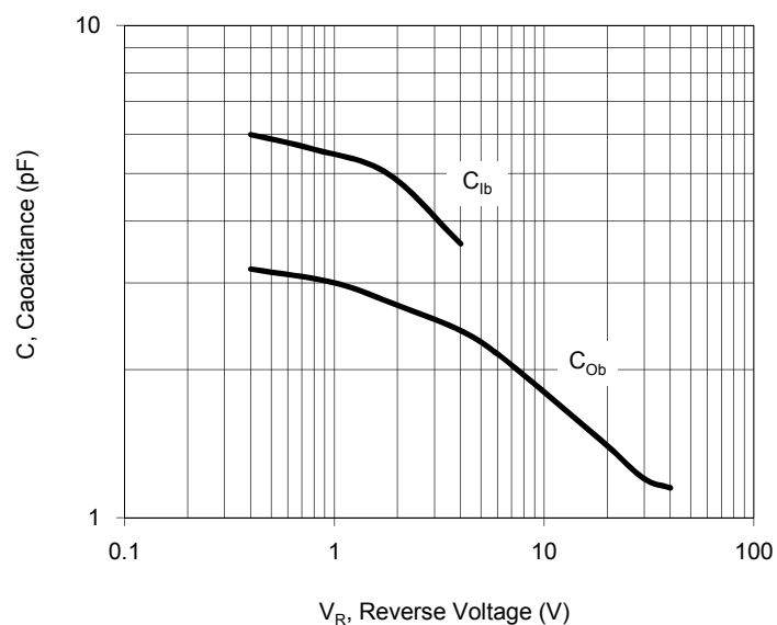
Fig.5 Capacitances
