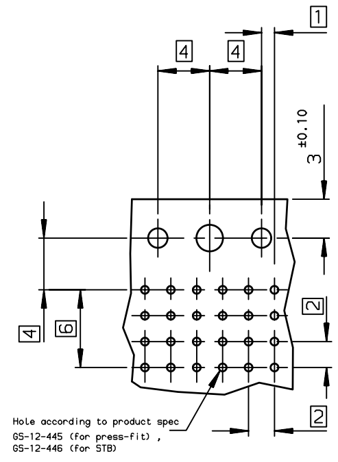
LAYOUT FOR P.C.B (PER 12mm LENGTH)
