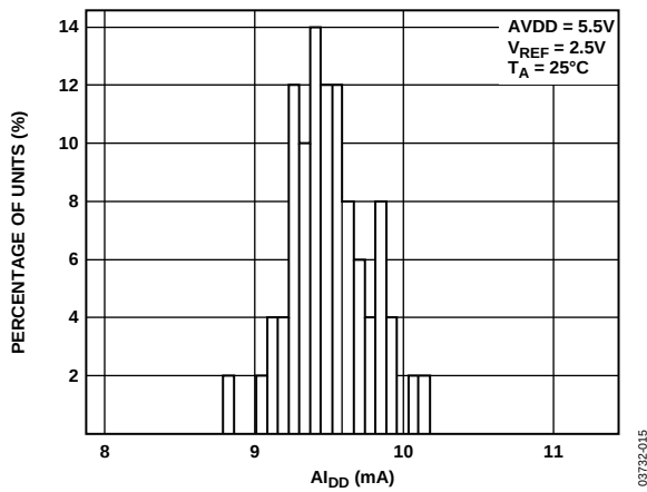
Figure 15. A_{IDDD} Histogram with Boost Off
