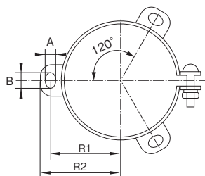
Code K (3—legs)
