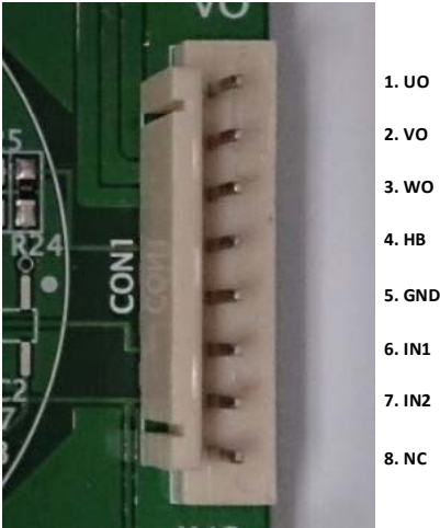
Figure 3. Pin header CON1
