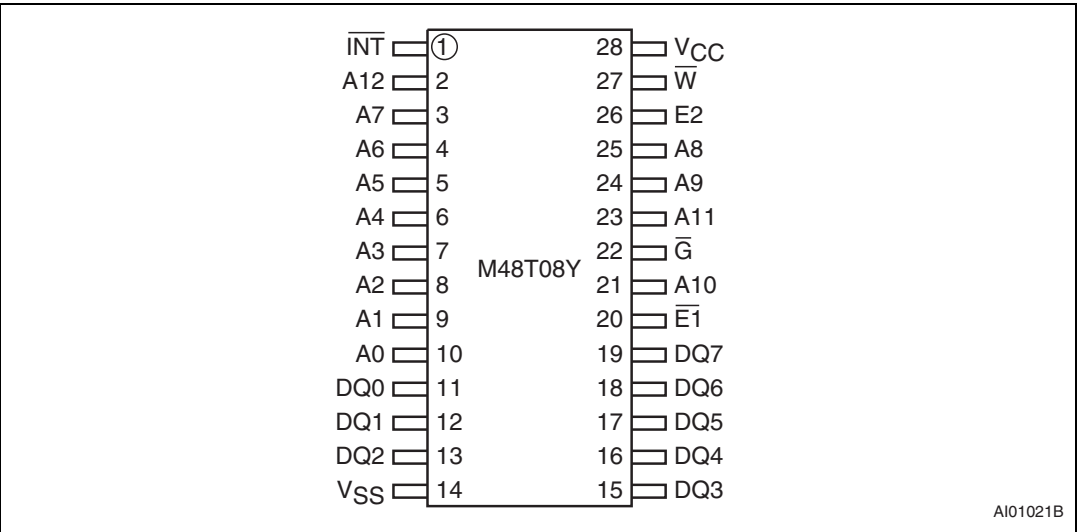
Figure 3. SOIC connections
