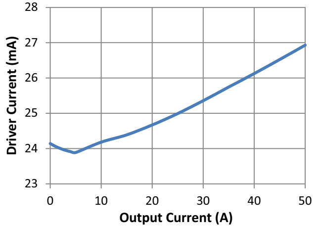
Figure 11. Driver Current vs. Output Current
