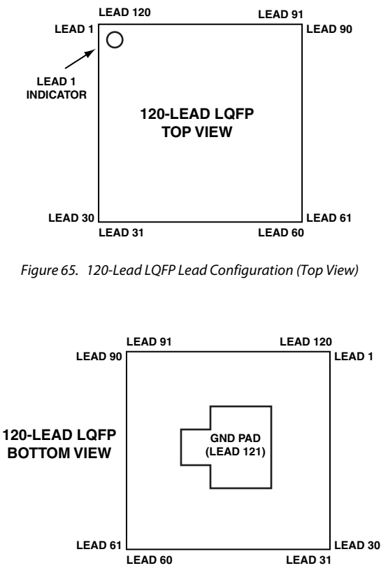
Figure 66. 120-Lead LQFP Lead Configuration (Bottom View)
