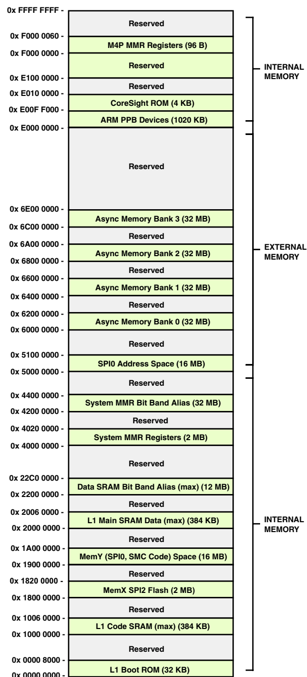
Figure 7. ADSP-CM40xF Memory Map
