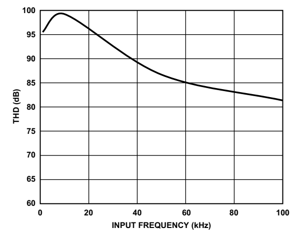
Figure 18. THD vs. Frequency, 0 V to 1.25 V Sine Wave Input
