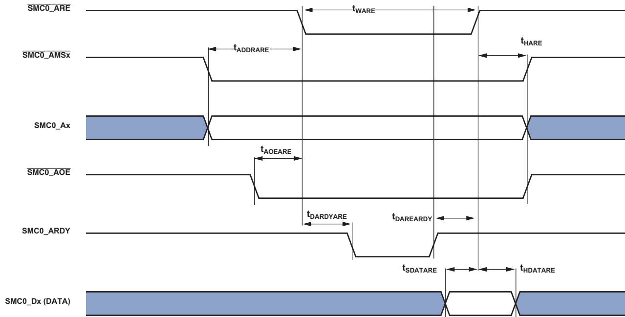
Figure 26. Asynchronous Read
