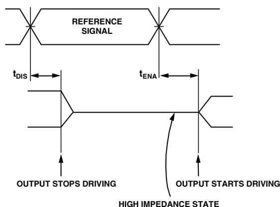
Figure 60. Output Enable/Disable
