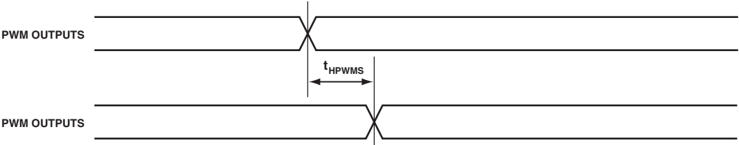
Figure 51. PWM Heightened-Precision Mode Timing, Output Skew
