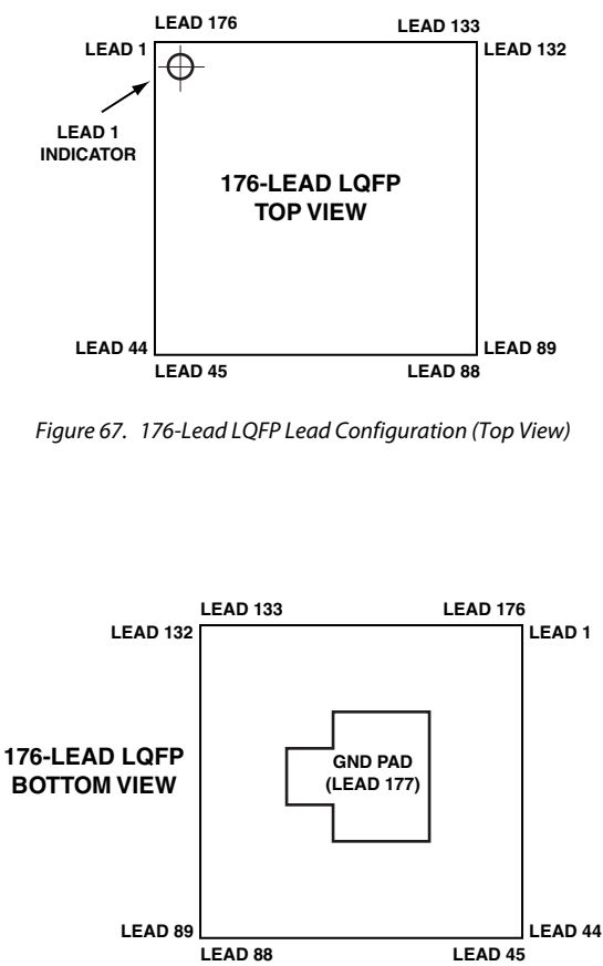
Figure 68. 176-Lead LQFP Lead Configuration (Bottom View)
