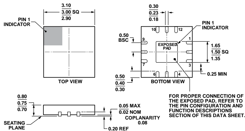
Figure 26. 12-Lead Lead Frame Chip Scale Package [LFCSP_WQ] 3 mm x 3 mm Body, Very Very Thin Quad (CP-12-5) Dimensions shown in millimeters
