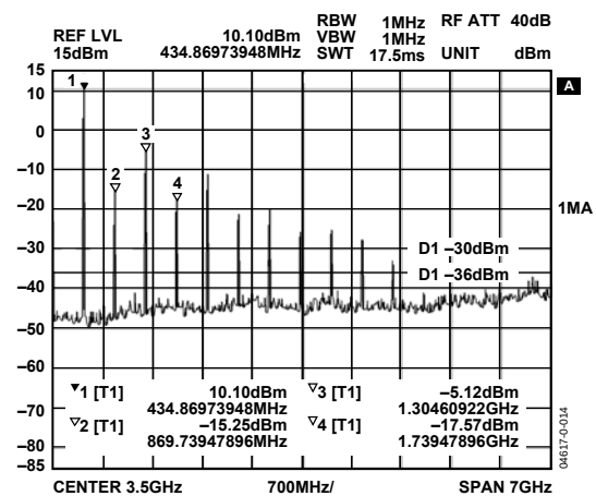
Figure 14. Harmonic Response, RF_{OUT} Matched to 50Ω, No Filter
