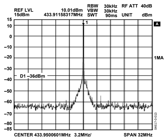
Figure 13. Spurious Components—Meets ETSI Specs
