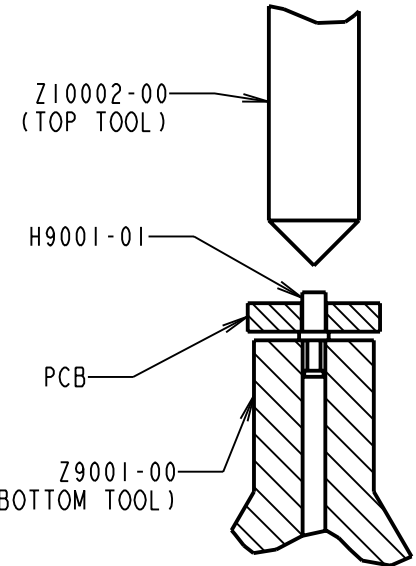
OPERATION DIAGRAM
