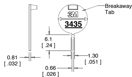
3435-0 Keying Plug (Optional: Order Separately)
