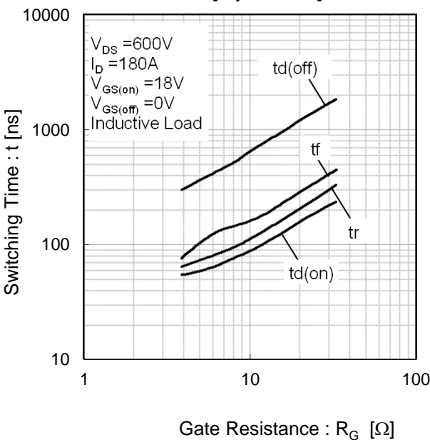
Fig.16 Switching Characteristics vs. Gate Resistance [ Tj=125°C ]
