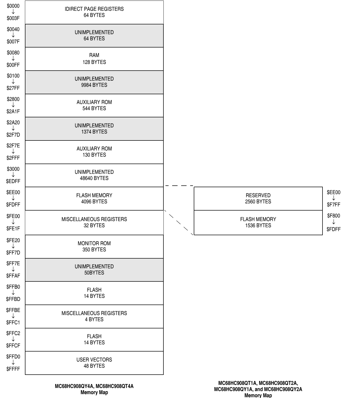
Figure 2-1. Memory Map
