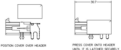
COVER ASSEMBLY METHOD
