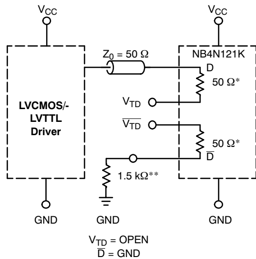
Figure 13. LVCMOS/LVTTL Interface
