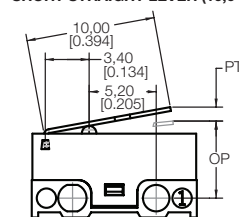
TYPE B SHORT STRAIGHT LEVER (10,0 mm)
