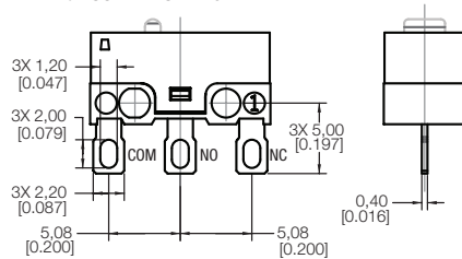
TYPE 50 - PCB RIGHT SIDE
