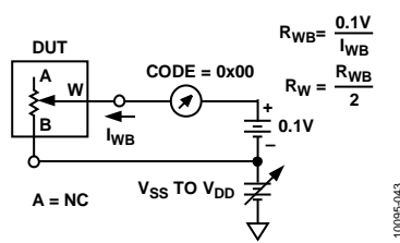
Figure 34. Wiper Resistance
