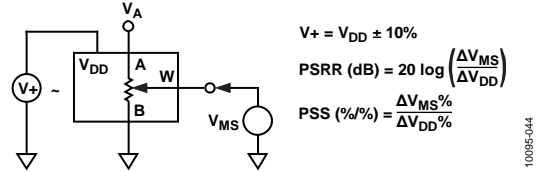
Figure 35. Power Supply Sensitivity (PSS, PSRR)
