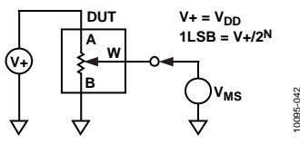
Figure 33. Potentiometer Divider Nonlinearity Error (INL, DNL)
